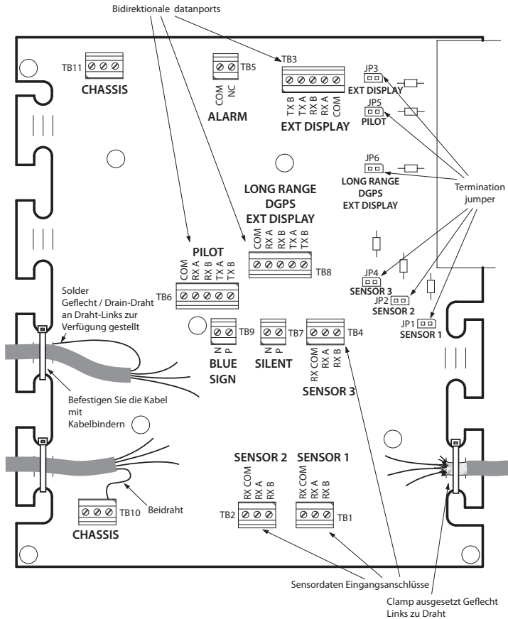
Abbildung 33 Junction-Box-Anschlüsse
